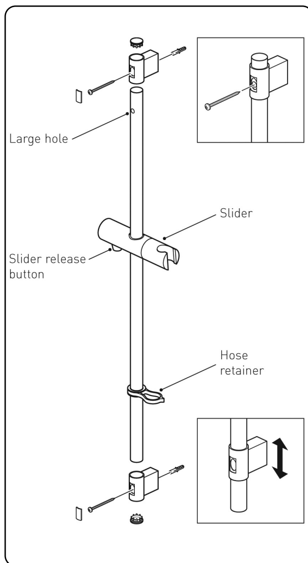
Figure 16: Fixing the riser rail
