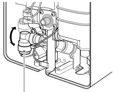
Fig 9a: Inlet connector elbow (left side, up, down or rear)
