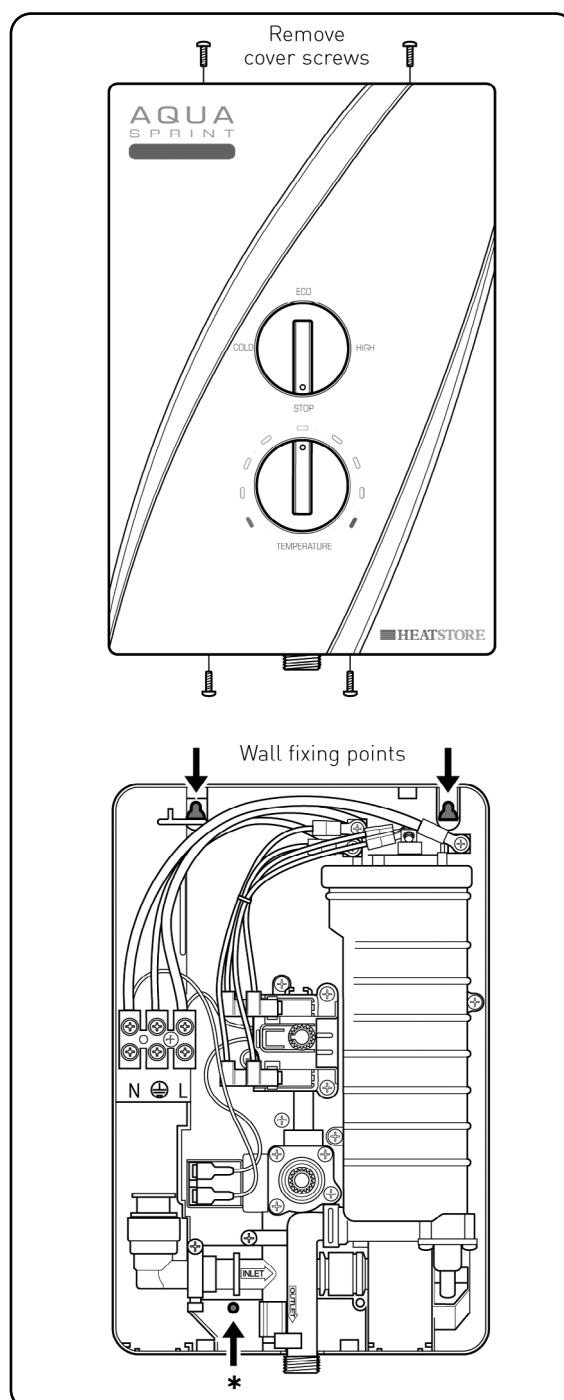
Figure 7: Removing the Cover
